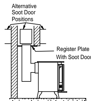
Fig. 9. Horizontal Register Plate With Rear Flue Connection
